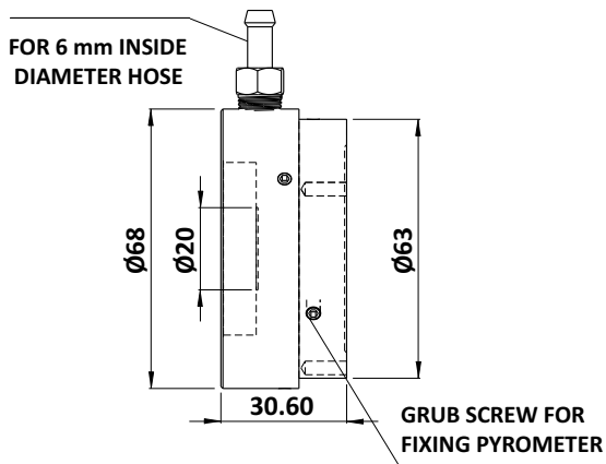
Air Purge Unit (Reference no: 8000-04)
