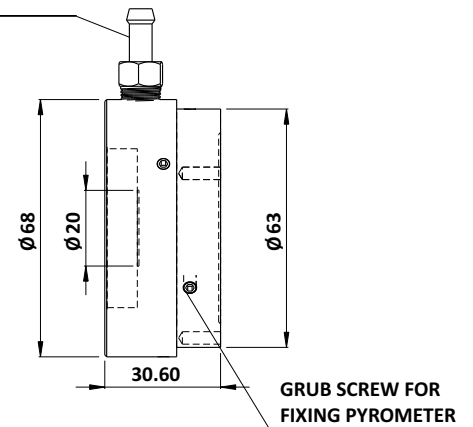
Air Purge Unit (Reference no: 8000-04)
