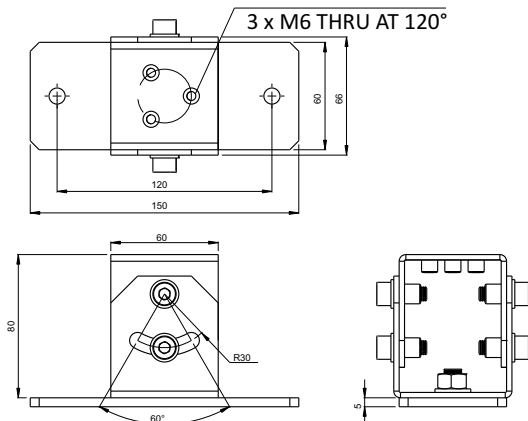
Adjustable Mounting Stand (Reference no: 8000-07)
